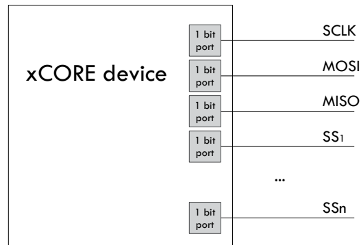
Figure 5: SPI master connection to the xCORE device
